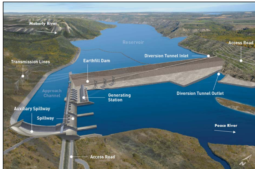
Figure 4. Artist's rendition of the Site C dam, generating station and spillways (BC Hydro 2013).
