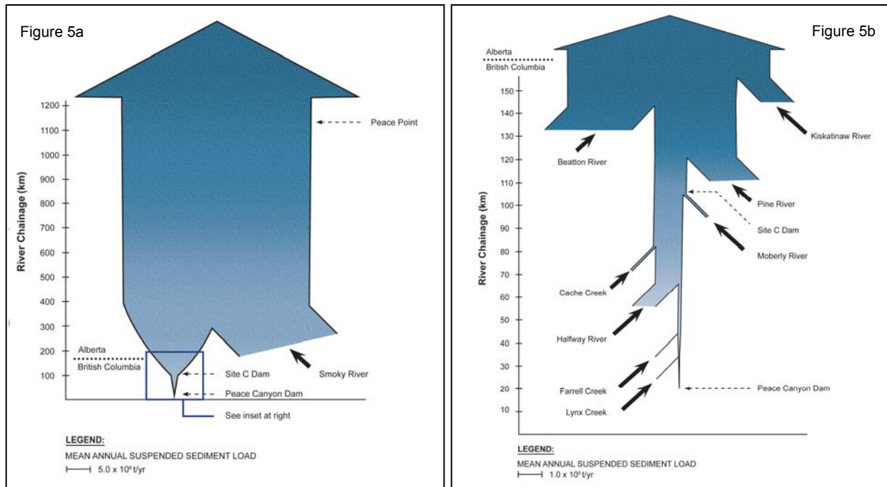
Figure 5. Peace River suspended sediment load.
