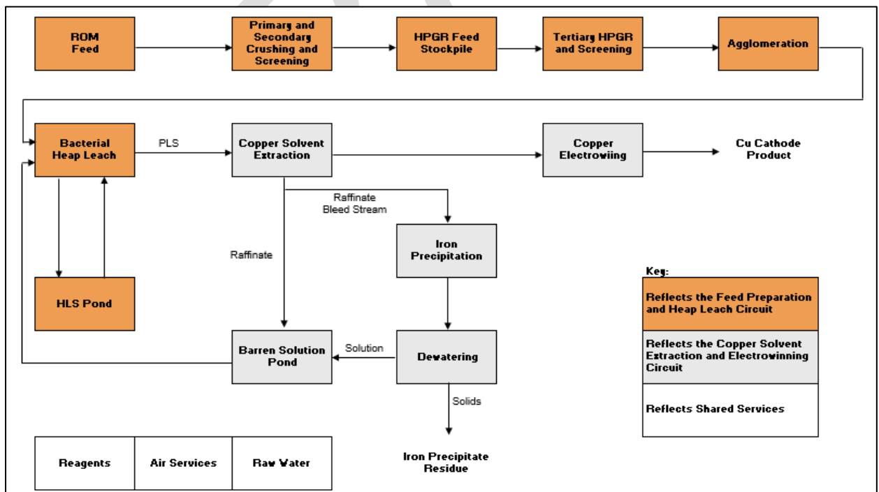
Figure 4-9: Hydrometallurgical Plant Simplified Summary Flowsheet
