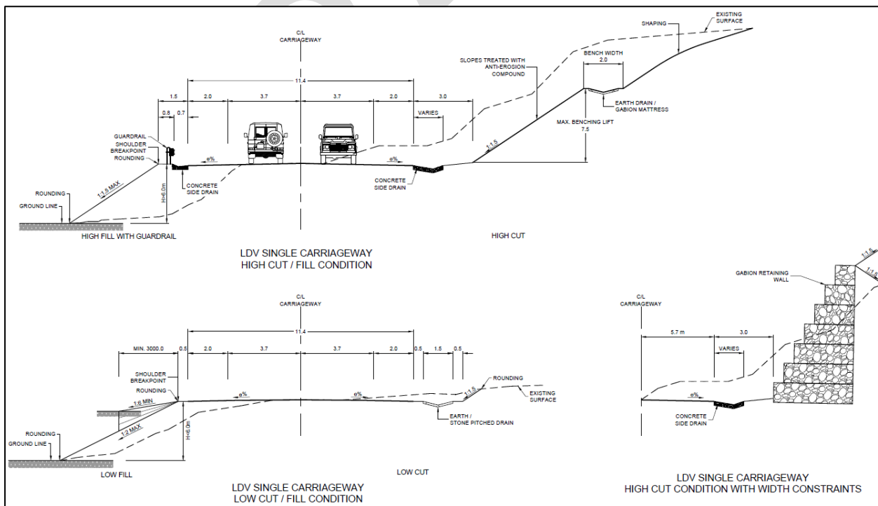
Figure 4-12: Typical section along the Project access route
