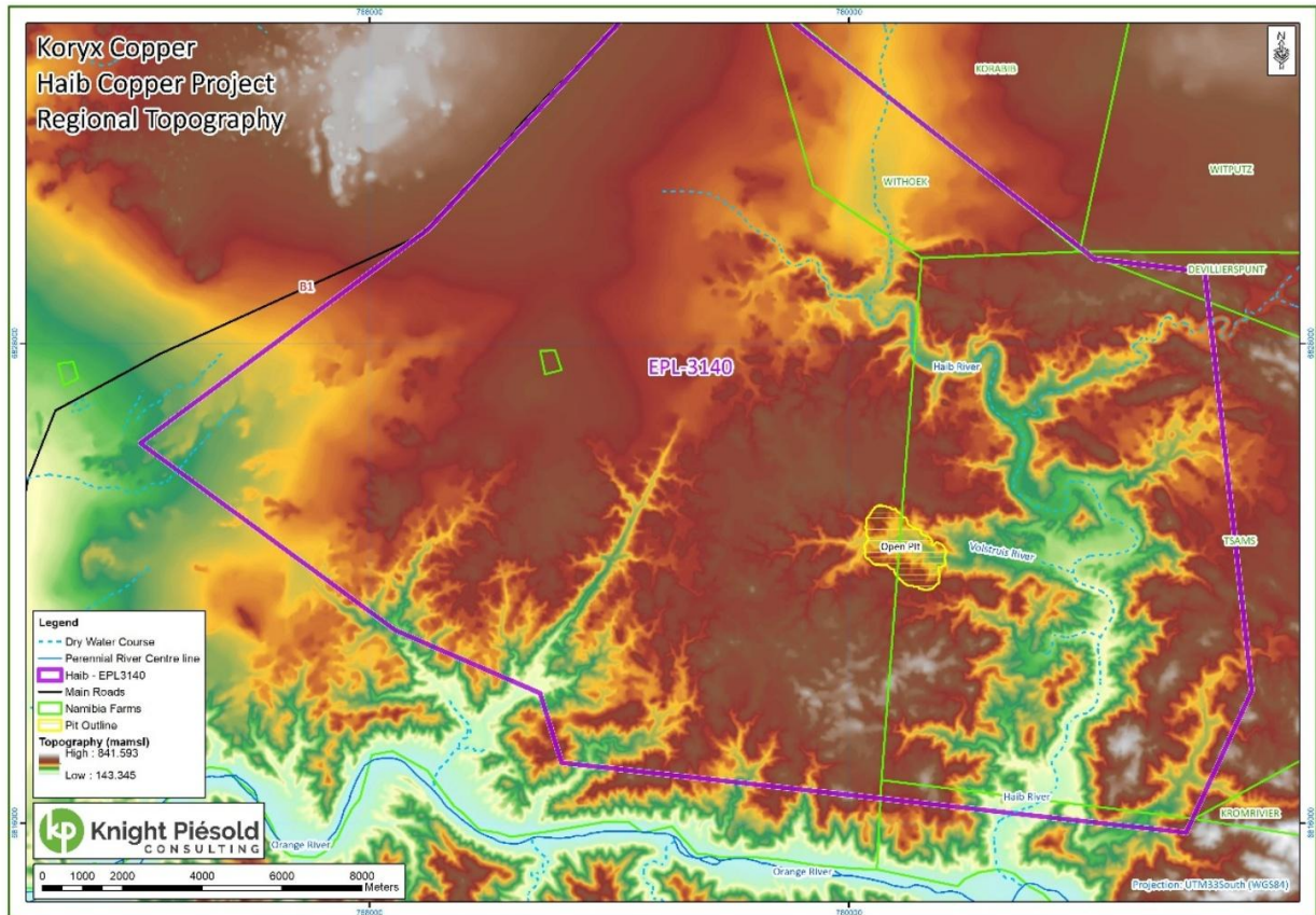
Figure 6-2: Regional topography
